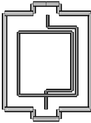
Figure 9-1: A square 1.75-turn RF inductor with an area of 2.25 \text{ mm}^2 and surrounded by a ground ring.
