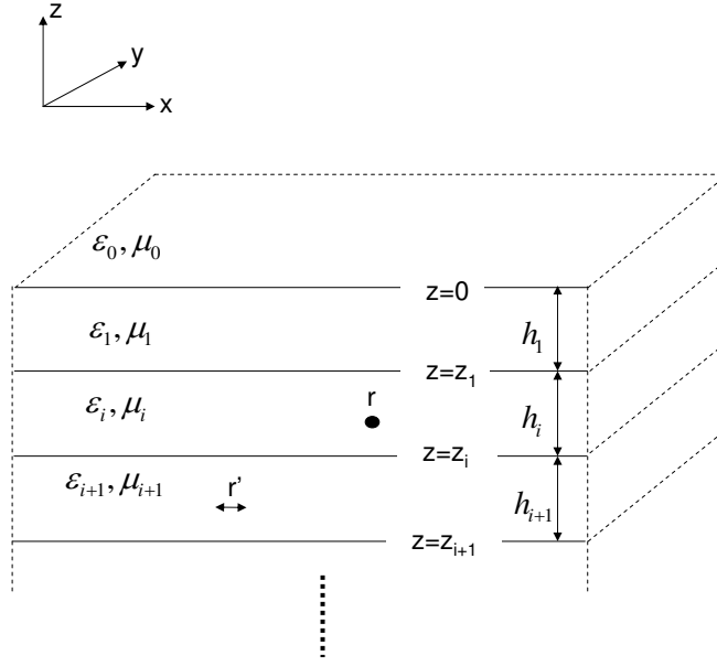
Figure 4-3: A source dipole and an evaluation point embedded in arbitrary layers of a multilayered planar medium.
