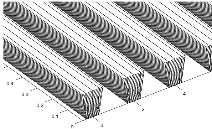
Figure 9-22: Structural view of an array of 8 conductors with trapezoidal cross-sections. Each conductor is 300\mu m in length with a cross-sectional dimension of 1.2\mu m in thickness, 1\mu m on the top base and 0.6\mu m on the bottom base. Separation distance between the conductors is 2\mu m .
