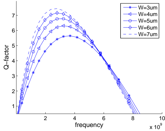
Figure 9-12: Quality factors for W=3\mu\text{m} , 4\mu\text{m} , 5\mu\text{m} , 6\mu\text{m} , 7\mu\text{m} ( SI=2\mu\text{m} , T=1\mu\text{m} , N=3 , OD=400\mu\text{m} ).
