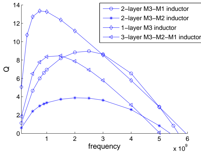
Figure 9-21: Quality factor analysis for the four inductors in Fig. 9-19.
