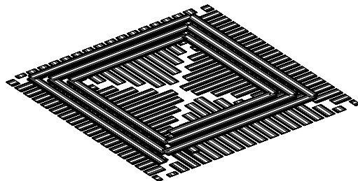
Figure 9-16: Angled view of a spiral inductor with a patterned ground shield.
