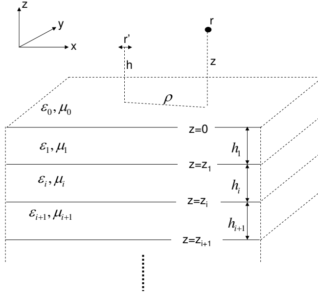
Figure 4-1: A source dipole and an evaluation point in the topmost layer of a multi-layered planar medium.
