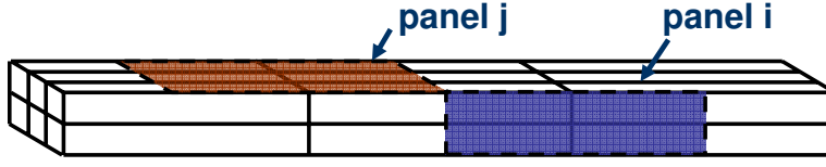
Figure 3-4: A conductor surface is discretized into panels so as to support current charge basis functions, where each basis function coefficient represents a panel charge [13].
