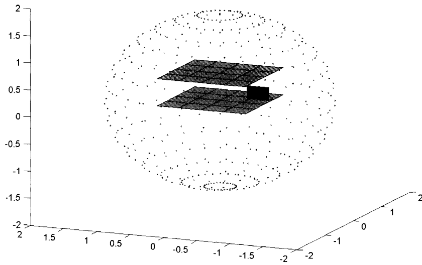
Figure 4-3: Three dimensional panel within its pFFT cell with surrounding collocation sphere
