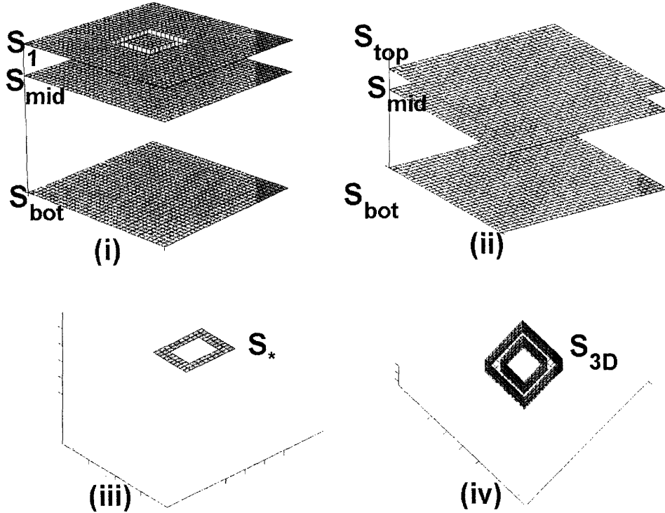
Figure 3-4: Breakdown of three-dimensional problem geometry into different components
