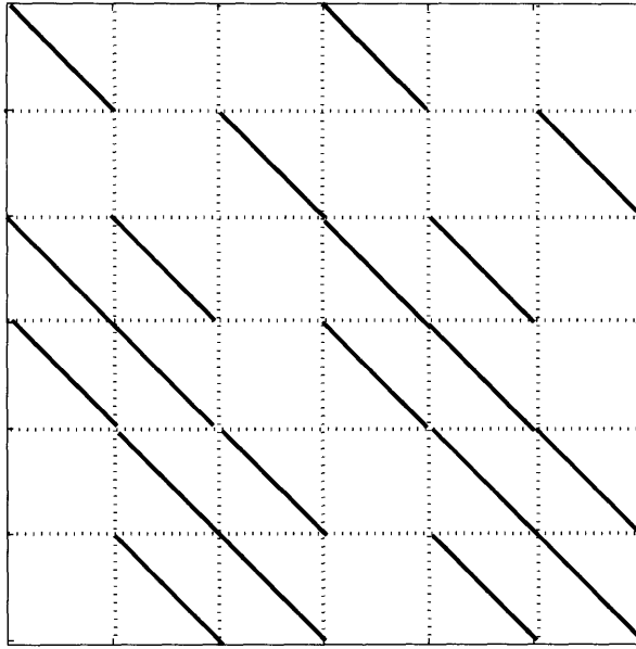
Figure 3-7: Preconditioner sparsity pattern for planar problem
